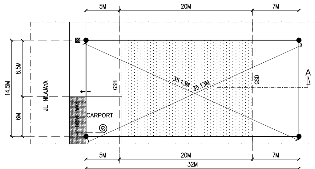
DENAH KAVLING JL. NILAJAYA NO. 25 SKALA 1 : 350
